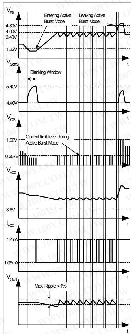
Figure 19 Signals in Active Burst Mode
