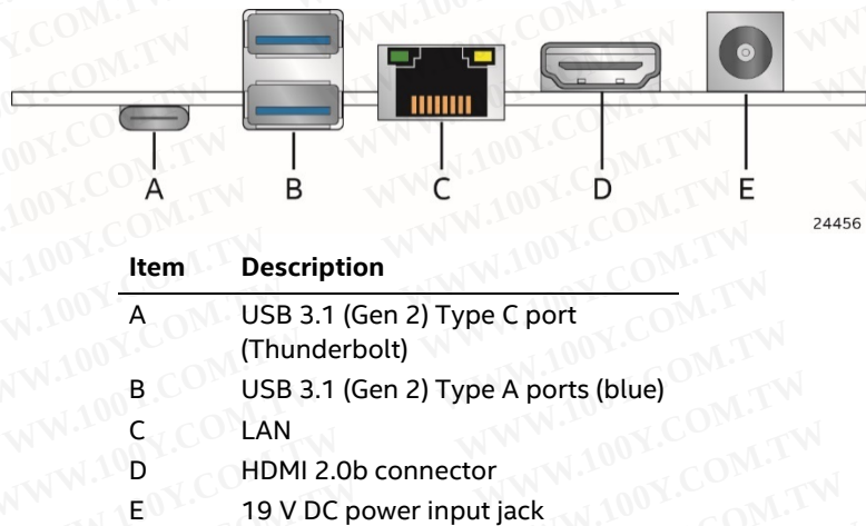
Figure 10. Back Panel Connectors
