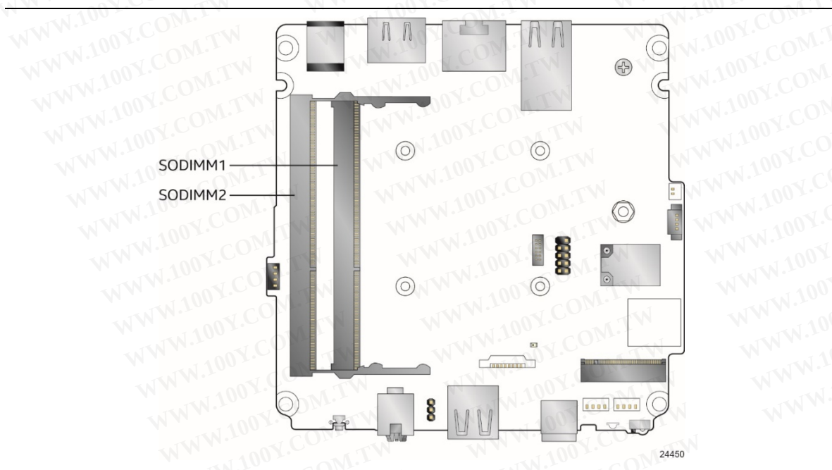
Figure 4. Memory Channel and SO-DIMM Configuration
