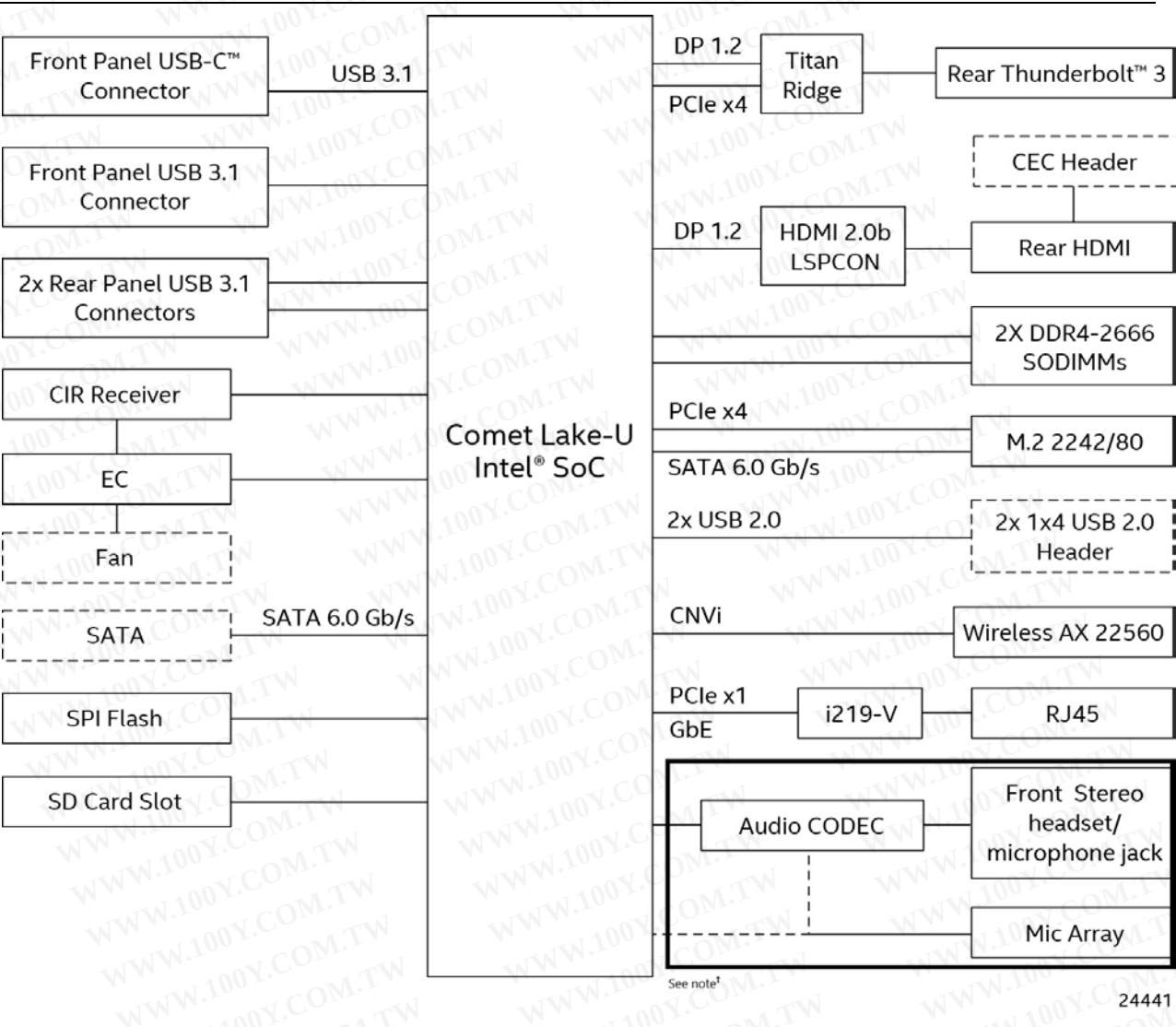
Figure 3. Block Diagram
