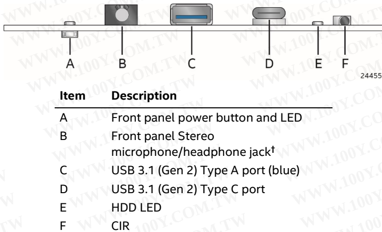
Figure 9. Front Panel Connectors
