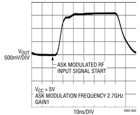
V_{OUT} Pulse Response, P_{IN} = 8dBm
