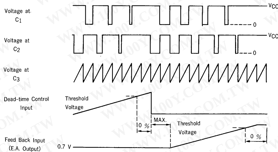
Voltage Waveform
