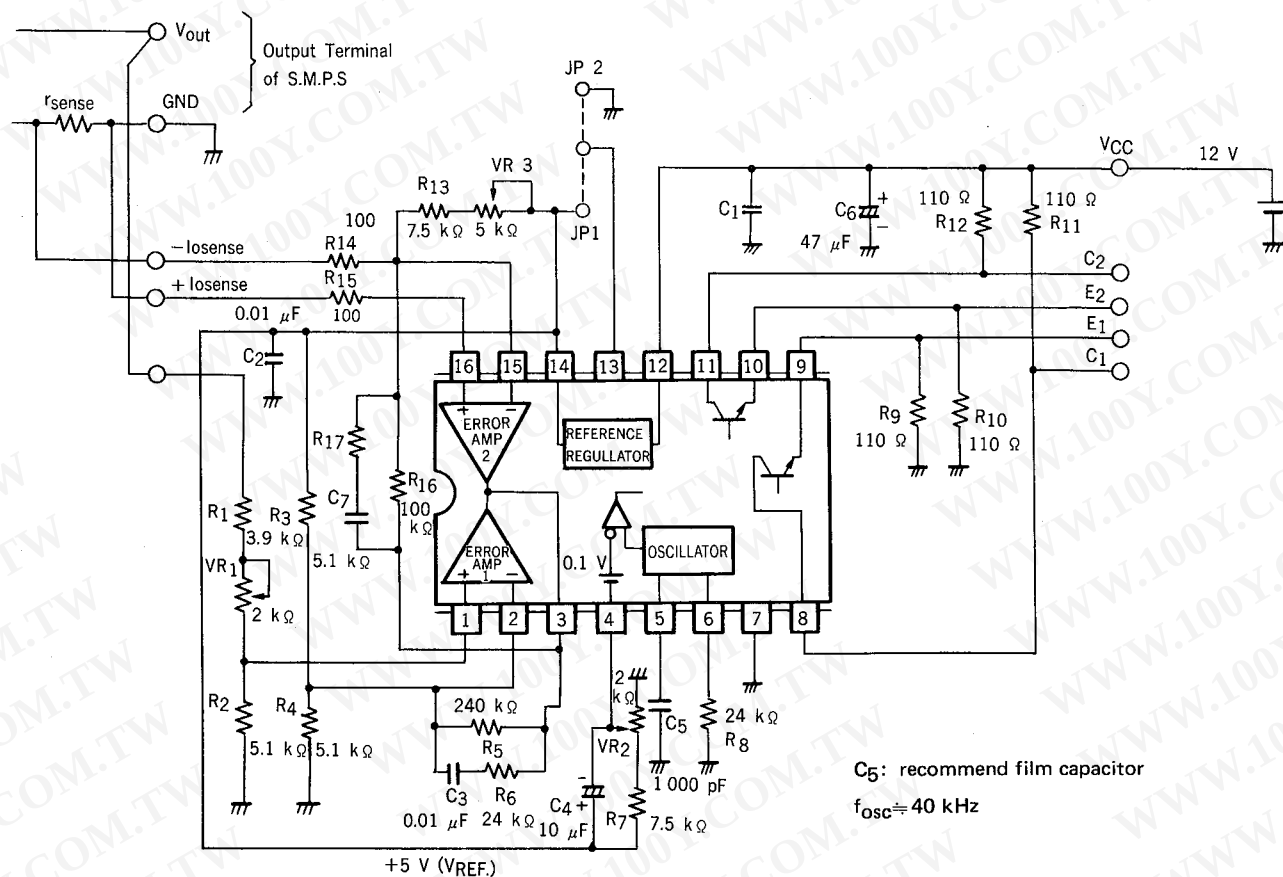
Fig. 2 Circuit
