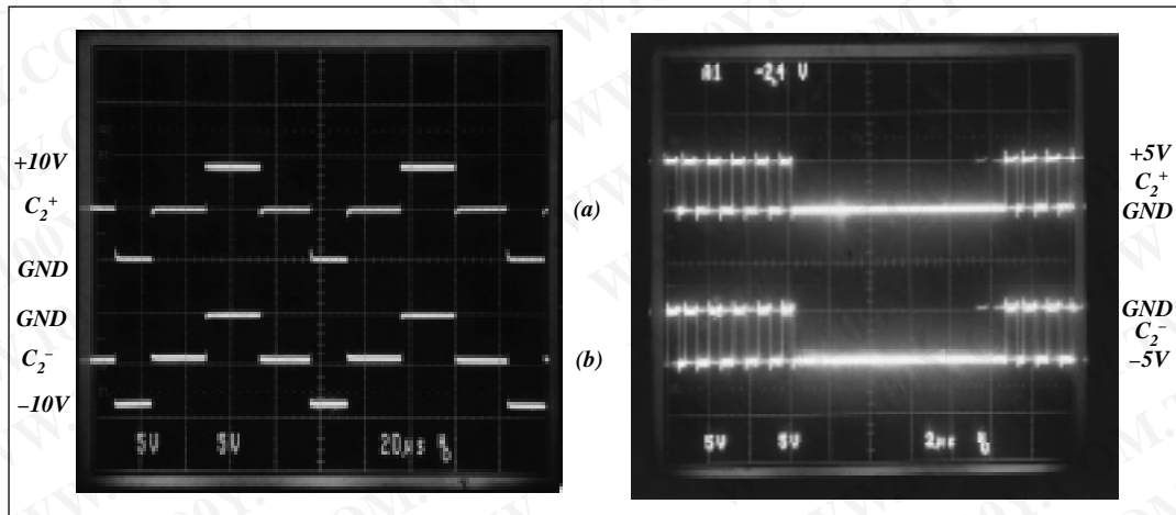
Figure 1. Charge Pump Waveforms
