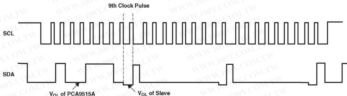
Figure 4. Bus 1 Waveforms
