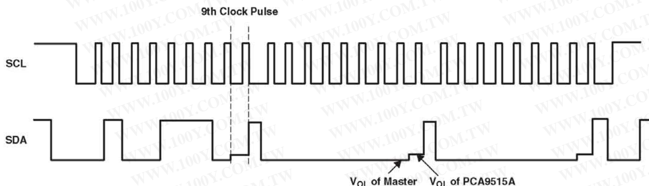
Figure 3. Bus 0 Waveforms
