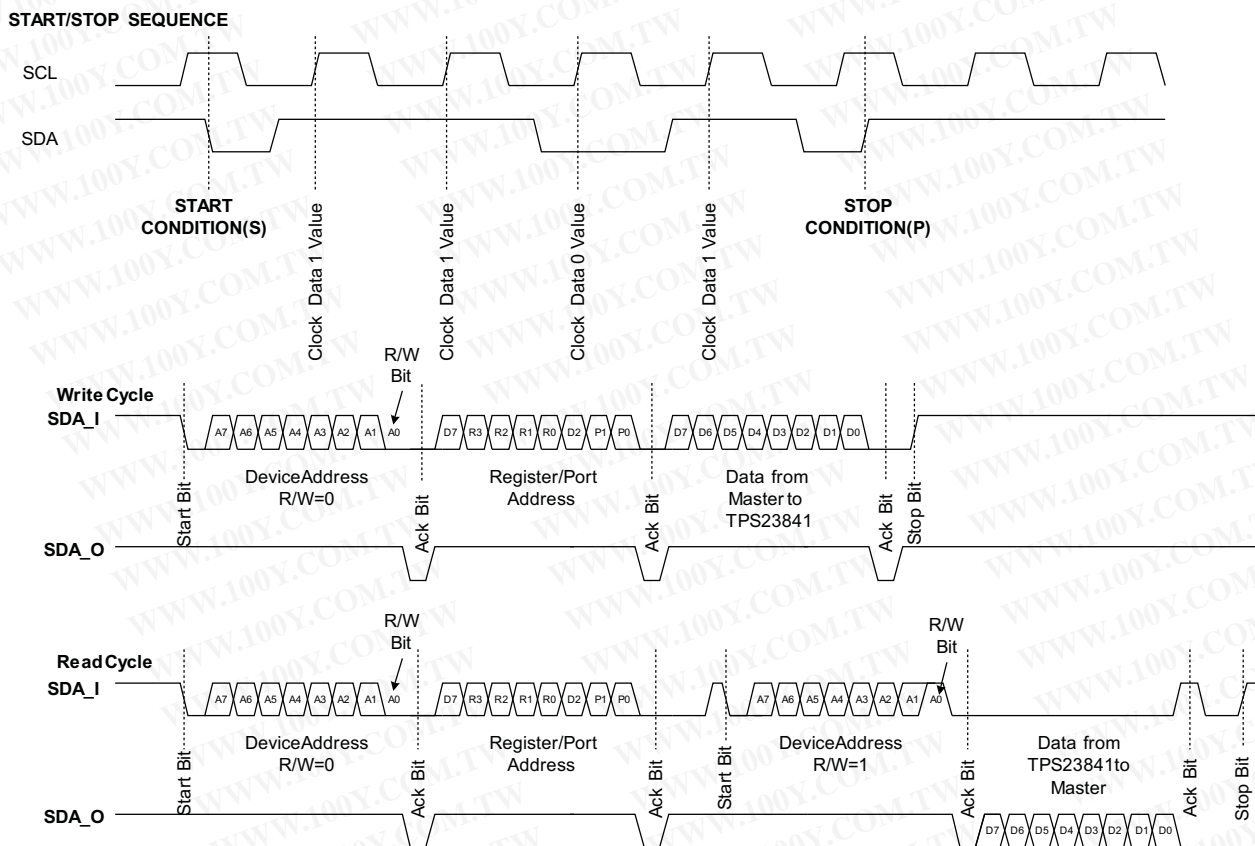
Figure 16. I²C Read/Write Cycles
