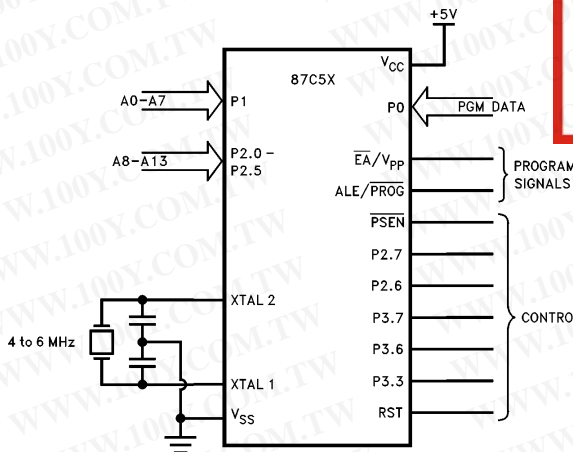
Figure 10. Programming the EPROM
