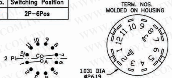
Schematic
