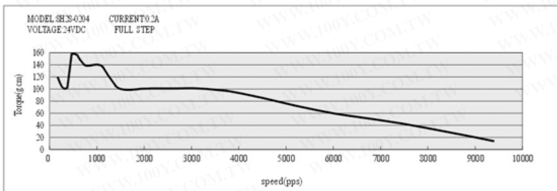
Pull out Torque Curve
