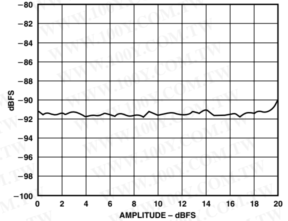
TPC 4. THD+N versus Amplitude at 1 kHz
