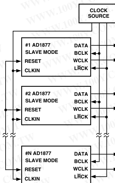
Figure 6. Synchronizing Multiple AD1877s
