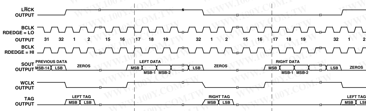
Figure 11. Serial Data Output Timing: Master Mode, Right-Justified with No MSB Delay, S_M = LO , RLJUST = HI , MSBDLY = HI
