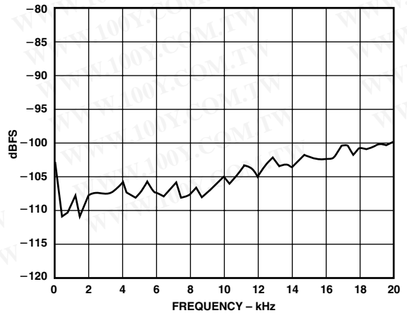
TPC 6. Channel Separation versus Frequency at -0.5 dBFS
