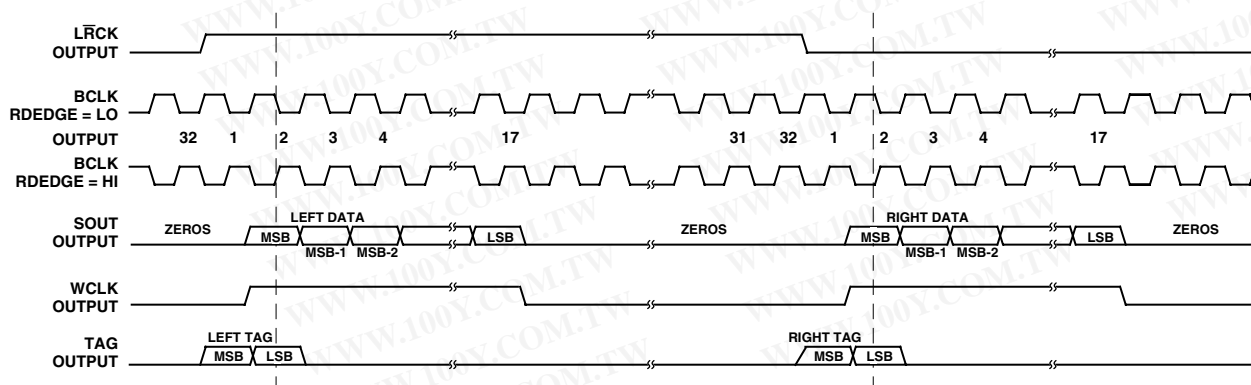
Figure 14. Serial Data Output Timing: Master Mode, I²S-Justified, \overline{S\overline{M}} = \text{LO} , \overline{R\overline{L}JUST} = \text{LO} , \overline{MSBDLY} = \text{LO}
