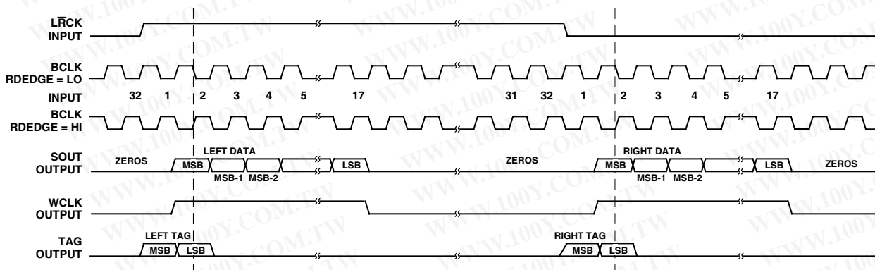
Figure 10. Serial Data Output Timing: Slave Mode, P_S -Justified, S_M = HI , RLJUST = LO , MSBDLY = LO
