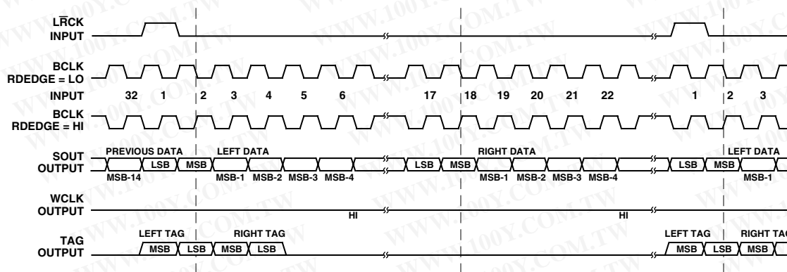
Figure 16. Serial Data Output Timing: Slave Mode, I^2S -Justified, 32-Bit Frame Mode, \overline{S}M = HI , RLJUST = LO , MSBDLY = LO
