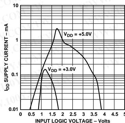
Figure 19. Supply Current vs. Logic Input Voltage
