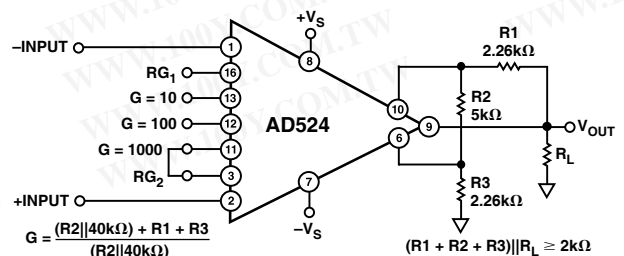
Figure 33. Gain of 2000
