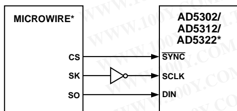
Figure 35. AD5302/AD5312/AD5322 to MICROWIRE Interface
