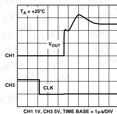
Figure 21. Exiting Power-Down to Midscale
