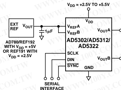
Figure 36. AD5302/AD5312/AD5322 Using External Reference
