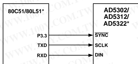
Figure 34. AD5302/AD5312/AD5322 to 80C51/80L51 Interface
