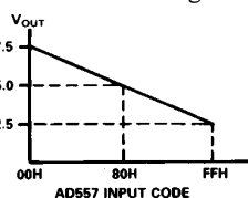
Figure 6. AD557 Input Code vs. Level Shifted Output in a "False" Ground Configuration
