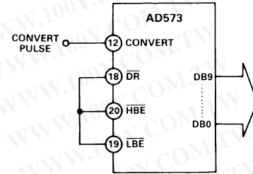
Figure 15. AD573 in “Stand-Alone” Mode (Output Data Valid 500 ns After DR Goes Low)
