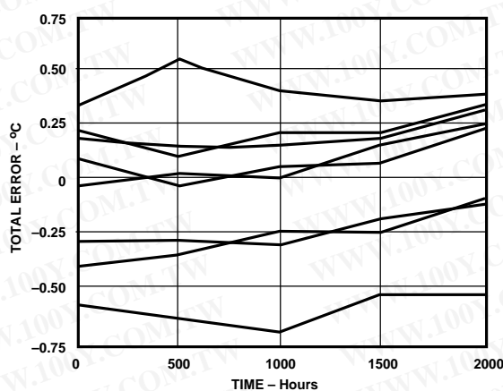
Long-Term Stability @ +85°C and 85% Relative Humidity
