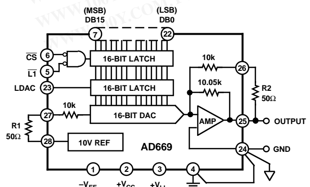
Figure 3a. 0 V to +10 V Unipolar Voltage Output
