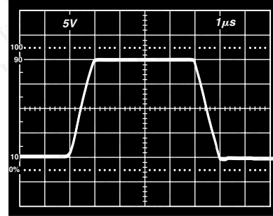
Figure 14. Transient Response R_L = 2 \text{ k}\Omega , C_L = 500 \text{ pF}
