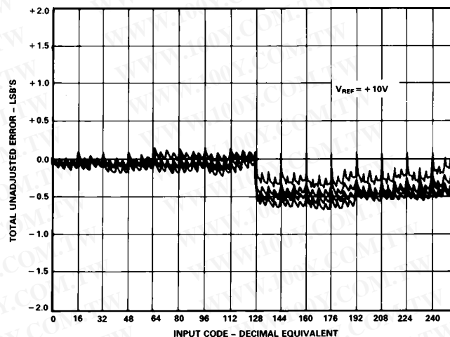
Figure 6. Channel-to-Channel Matching
