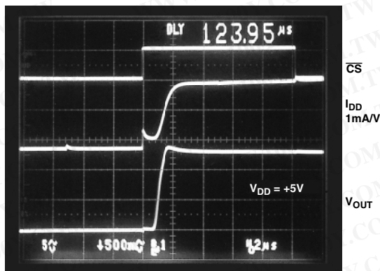
Figure 16. Shutdown Recovery Time (Wakeup)
