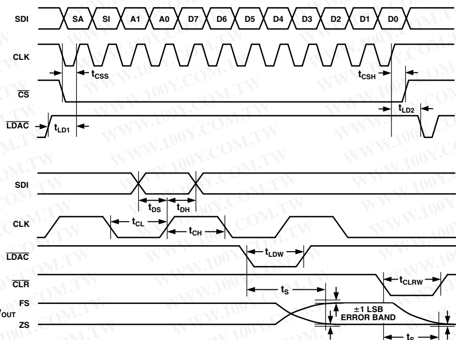
Figure 2. AD7304 Timing Diagram
