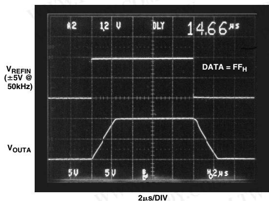
Figure 13. Multiplying Mode Step Response and Output Slew Rate
