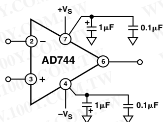
Figure 24. Recommended Power Supply Bypassing
