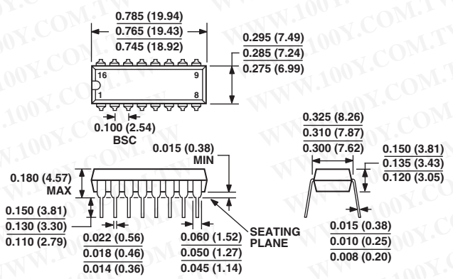
16-Lead Plastic Dual In-Line Package [PDIP] (N-16)
