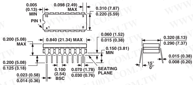
16-Lead Ceramic Dual In-Line Package [CERDIP] (Q-16)
