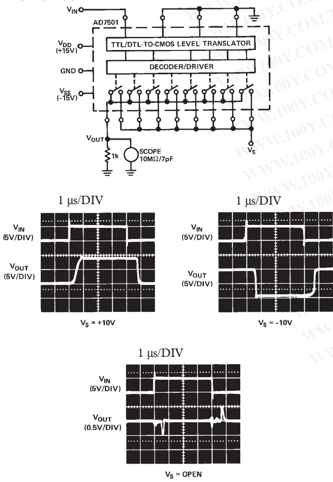
TEST CIRCUIT 2
