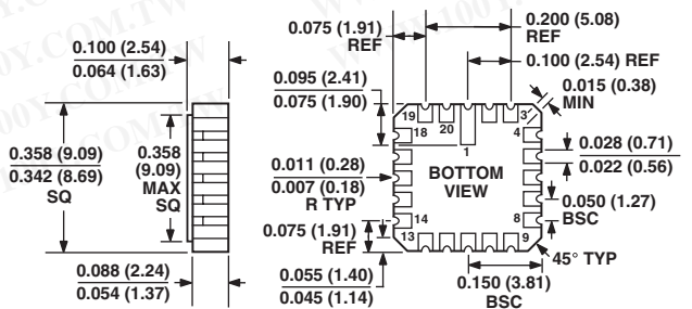
20-Terminal Ceramic Leadless Chip Carrier [LCC] (E-20A)
