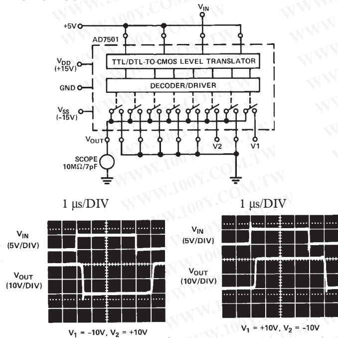
TEST CIRCUIT 1
