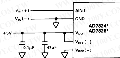
*ADDITIONAL PINS OMITTED FOR CLARITY, ONLY CHANNEL 1 SHOWN
