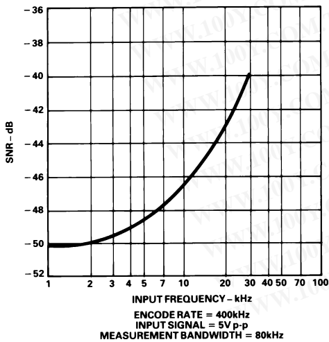
TPC 3. Signal-Noise Ratio vs. Input Frequency
