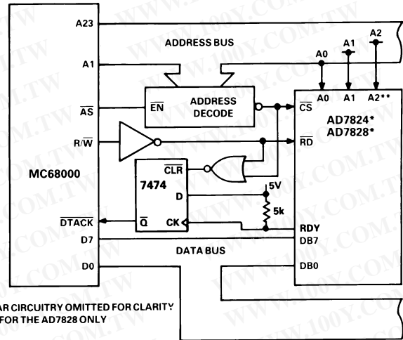
Figure 17. AD7824/AD7828-MC68000 Interface
