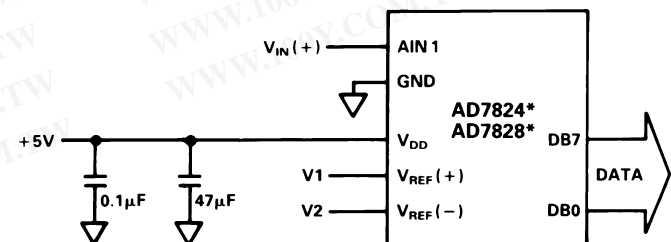
*ADDITIONAL PINS OMITTED FOR CLARITY, ONLY CHANNEL 1 SHOWN
