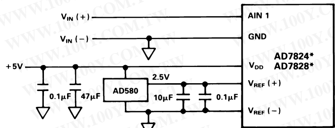
*ADDITIONAL PINS OMITTED FOR CLARITY, ONLY CHANNEL 1 SHOWN
