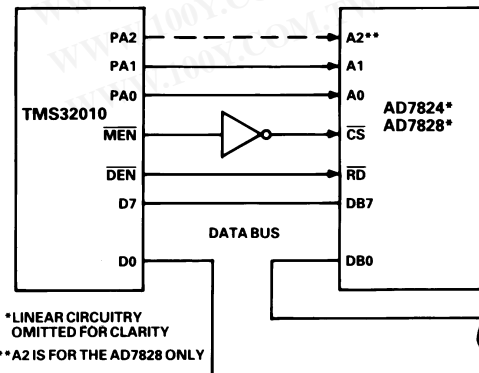
Figure 18. AD7824/AD7828-TMS32010 Interface
