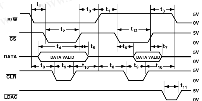
Figure 3. Timing Diagram
