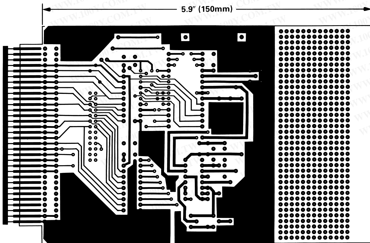
Figure 30. PCB Solder Side Layout for Figure 30
