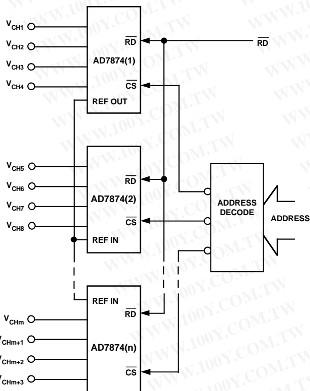
Figure 18. Multiple AD7874s in Multichannel System
