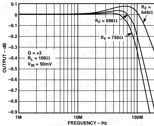
Figure 11. 0.1\text{ dB} Flatness, R Package (for N Package Add 50\ \Omega to R_F )
