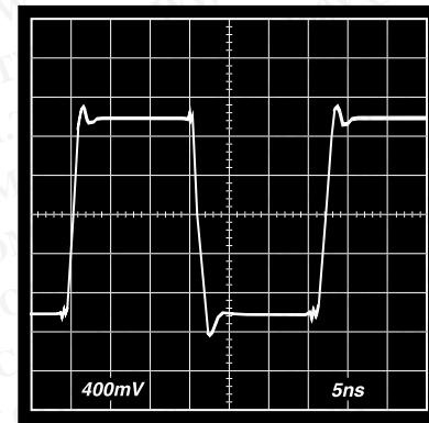
Figure 38. 2 V Step Response, G = -1
