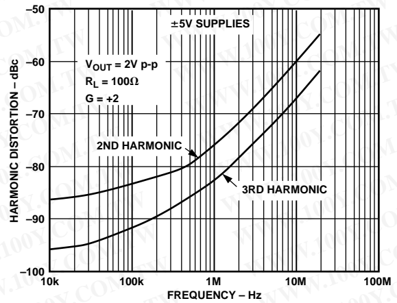
Figure 14. Distortion vs. Frequency, R_L = 100\ \Omega
