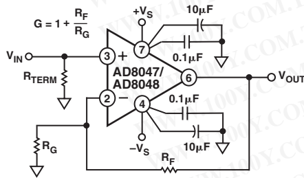
Figure 3. Noninverting Operation
