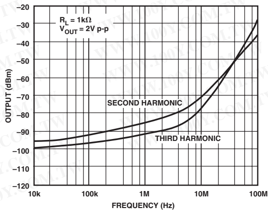
TPC 18. AD8047 Harmonic Distortion vs. Frequency, G = +1
