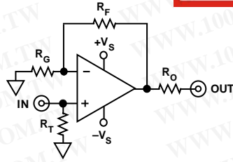
Noninverting Configuration
