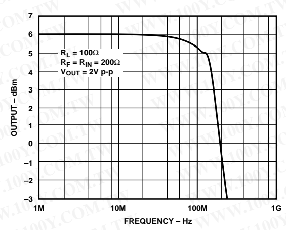
Figure 30. AD8048 Large Signal Frequency Response, G = +2
