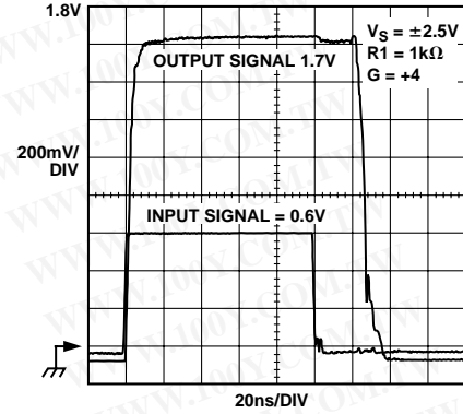
Figure 30. Output Overload Recovery, V_S = \pm 2.5\text{ V}
