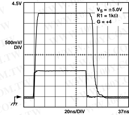
Figure 31. Output Overload Recovery, V_S = \pm 5.0\text{ V}
