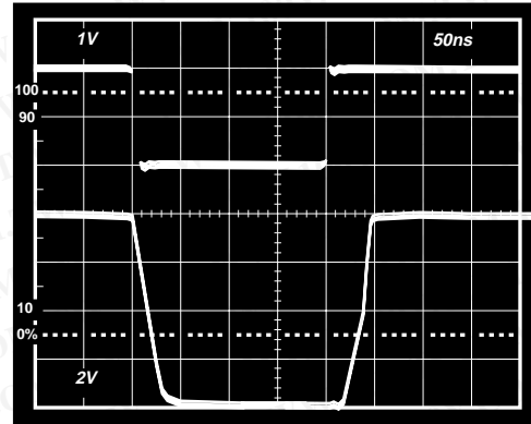
Figure 45. 6 dB Overload Recovery, G = +10 , ( R_L = 500 \Omega , R_F = 357 \Omega , V_S = \pm 5 V )
