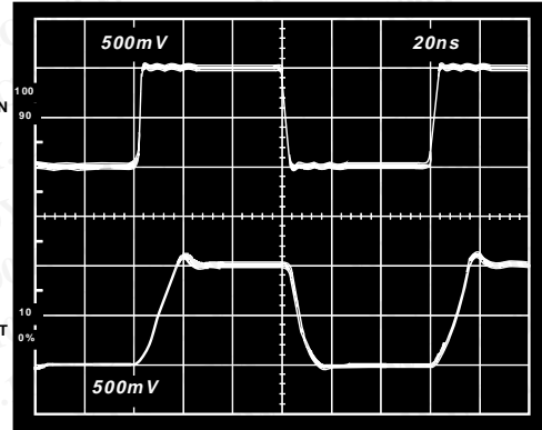
Figure 26. Small Signal Pulse Response, Gain = +1, ( R_F = 750\ \Omega , R_L = 150\ \Omega , V_S = \pm 5\ V )
