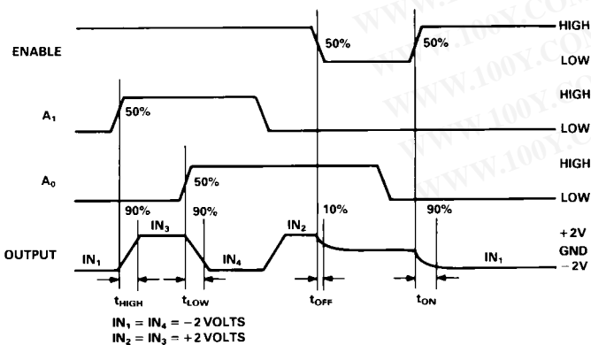
AD9300 Timing Diagram
