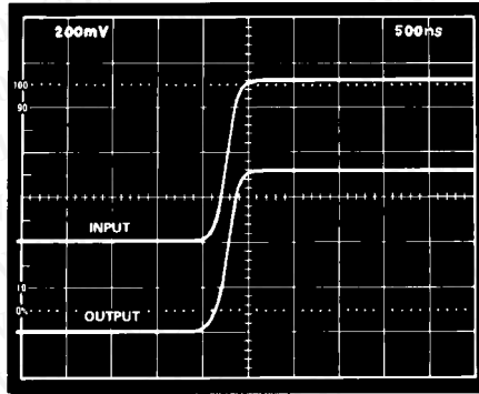
Figure 9. T-Step Response
