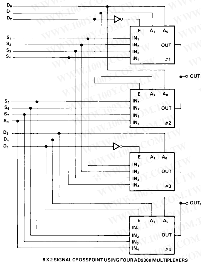
Figure 11. 8 \times 2 Signal Crosspoint Using Four AD9300 Multiplexers
