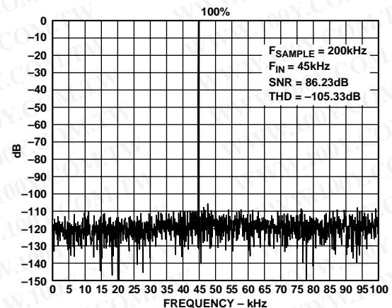
Figure 10. FFT PLOT
