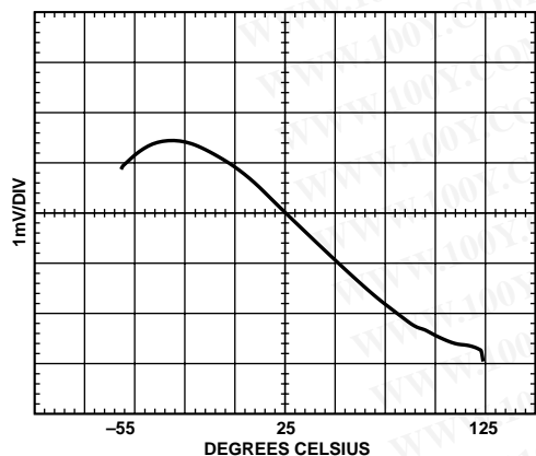
Figure 13. Reference Drift
