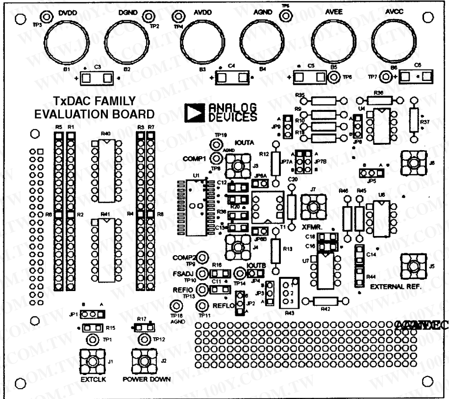
Figure 60. Silkscreen Layer—Top
