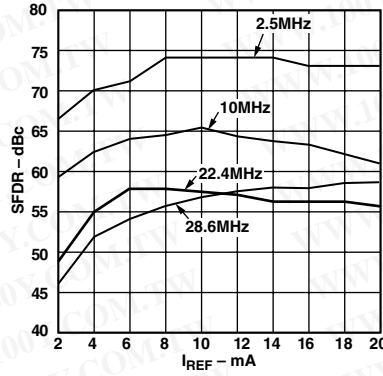
Figure 31. SFDR vs. f_{OUT} and I_{OUTFS} @ 100 MSPS, 0 dBFS
