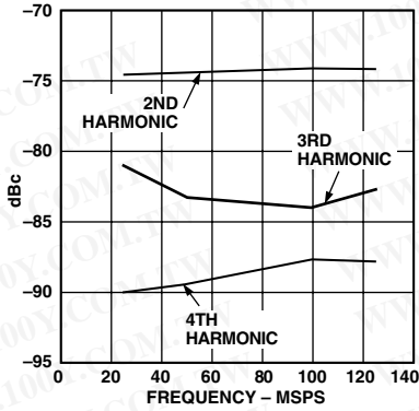
Figure 30. THD vs. f_{CLOCK} f_{OUT} = 2 \text{ MHz}
