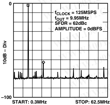
Figure 36. Single-Tone SFDR
