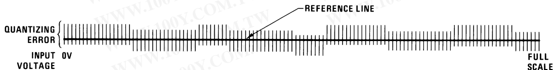
FIGURE 4. Typical Error Curve
