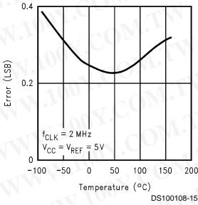
Linearity Error (TUE) vs Temperature
