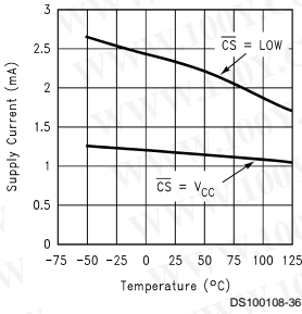
Power Supply Current vs Temperature (ADC08832)
