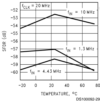
SFDR vs Temp and f_{IN}
