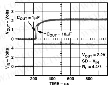
Figure 10. Power-Up Response
