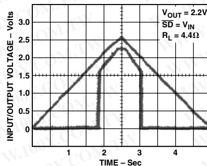
Figure 9. Power-Up/Power-Down
