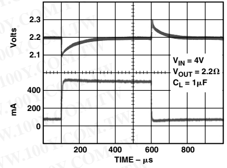
Figure 13. Load Transient Response
