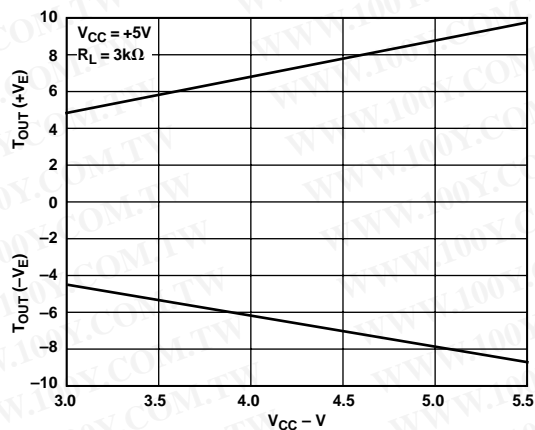
Figure 15. Transmitter Output Voltage vs. V_{CC}
