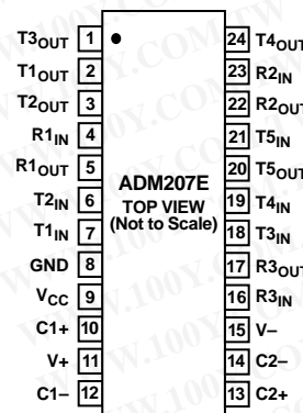
Figure 3. ADM207E Pin Configuration
