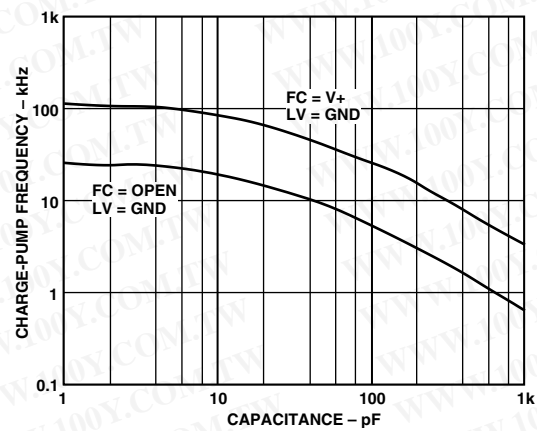
TPC 11. Charge-Pump Frequency vs. External Capacitance
