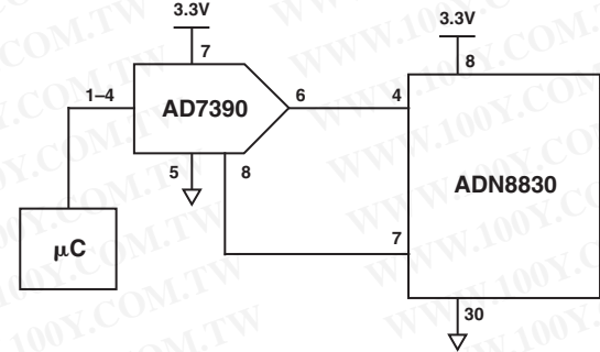
Figure 4. Using a DAC to Control the Temperature Setpoint
