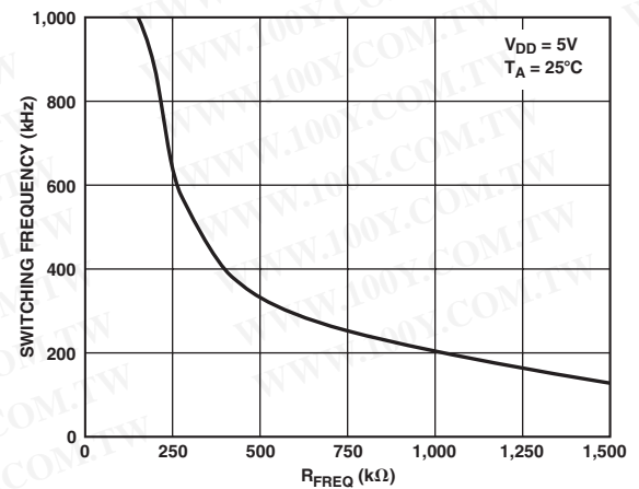
TPC 6. Switching Frequency vs. R REQ
