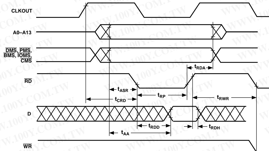
Figure 11. Memory Read
