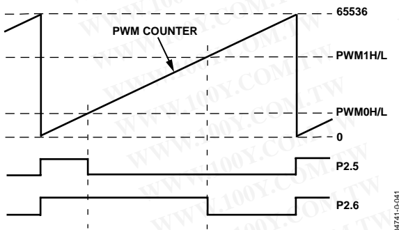
Figure 41. PWM Mode 3
