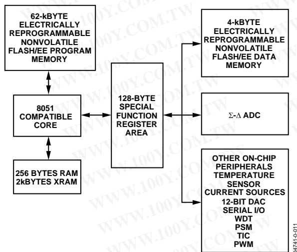
Figure 11. Programming Model
