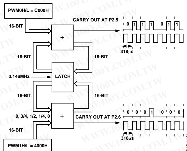
Figure 44. PWM Mode 6
