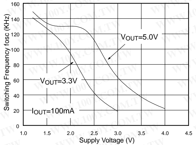
Fig. 22 Switching Frequency vs. Supply Voltage
