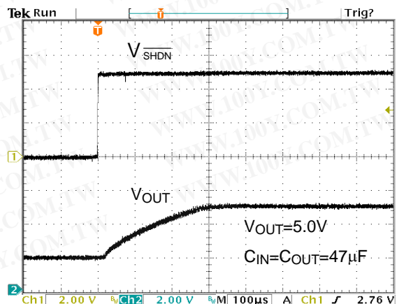
Fig. 30 Exiting Shutdown
