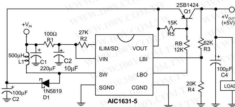
Fig. 5 4-Cell Input Step-Up / Step-Down Converter
