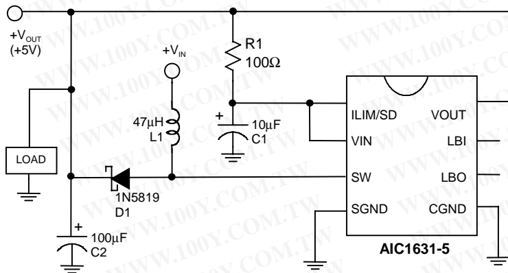
Fig. 4 1-Cell Input 5V Output Step-Up Converter
