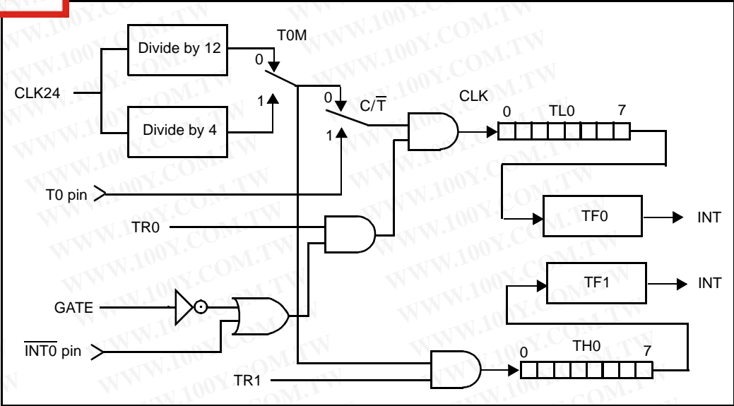
Figure C-3. Timer 0 - Mode 3
