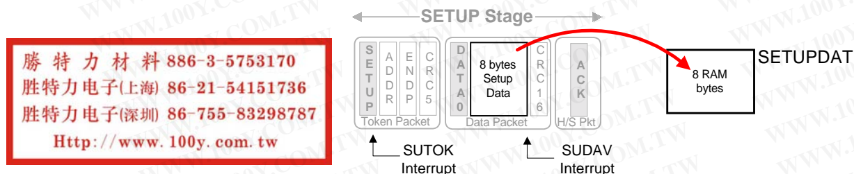
Figure 7-2. The Two Interrupts Associated with EP0 CONTROL Transfers
