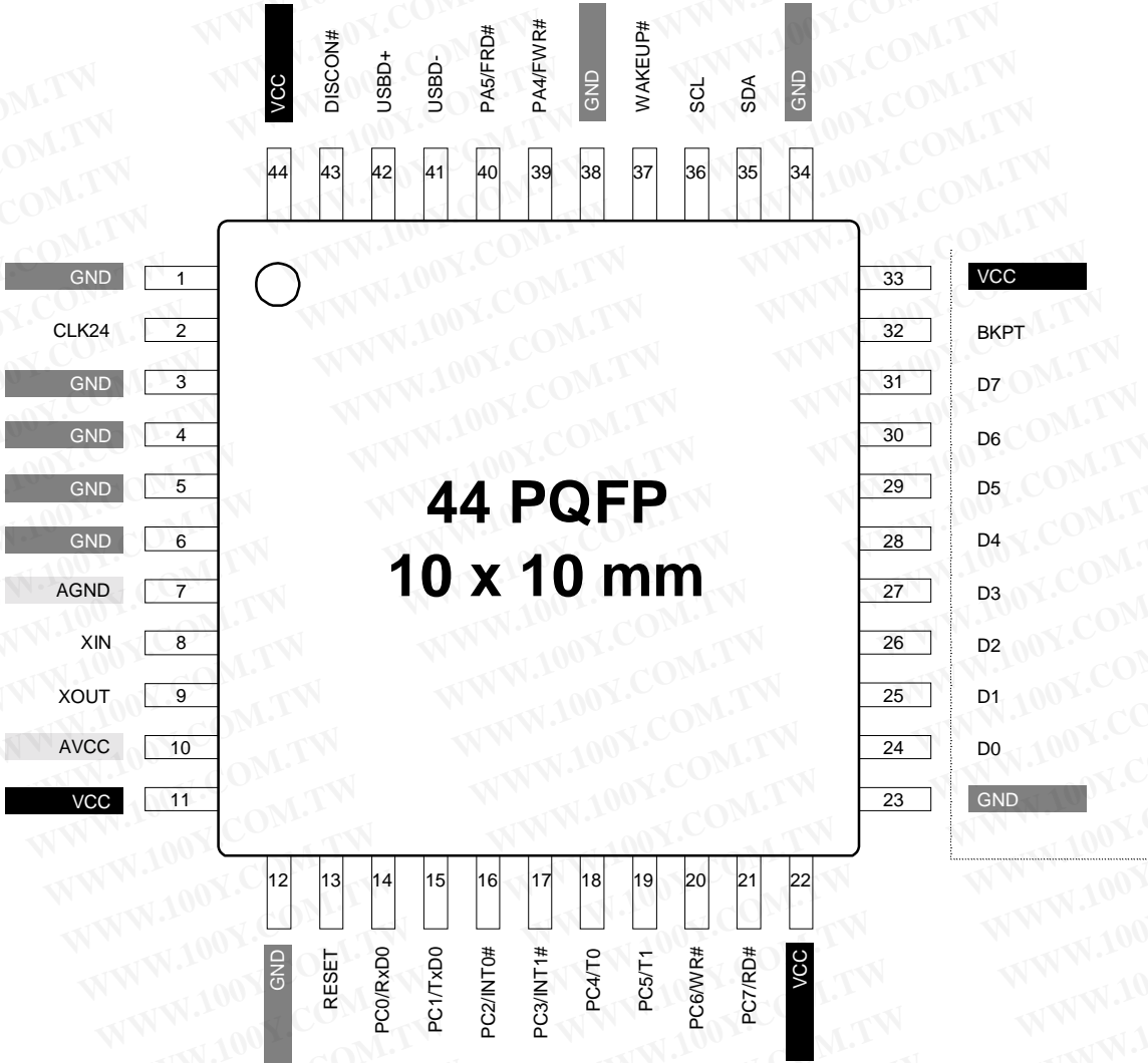
Figure 1-11. 44-pin Package with Data Bus (AN2135, and AN2136)
