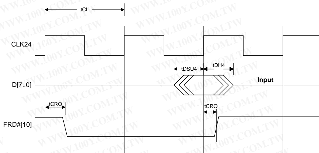
Figure 13-10. Fast Transfer Read Timing [Mode 10]
