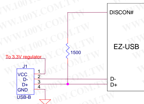
Figure 5-3. Typical Disconnect Circuit (DISCOE=1)
