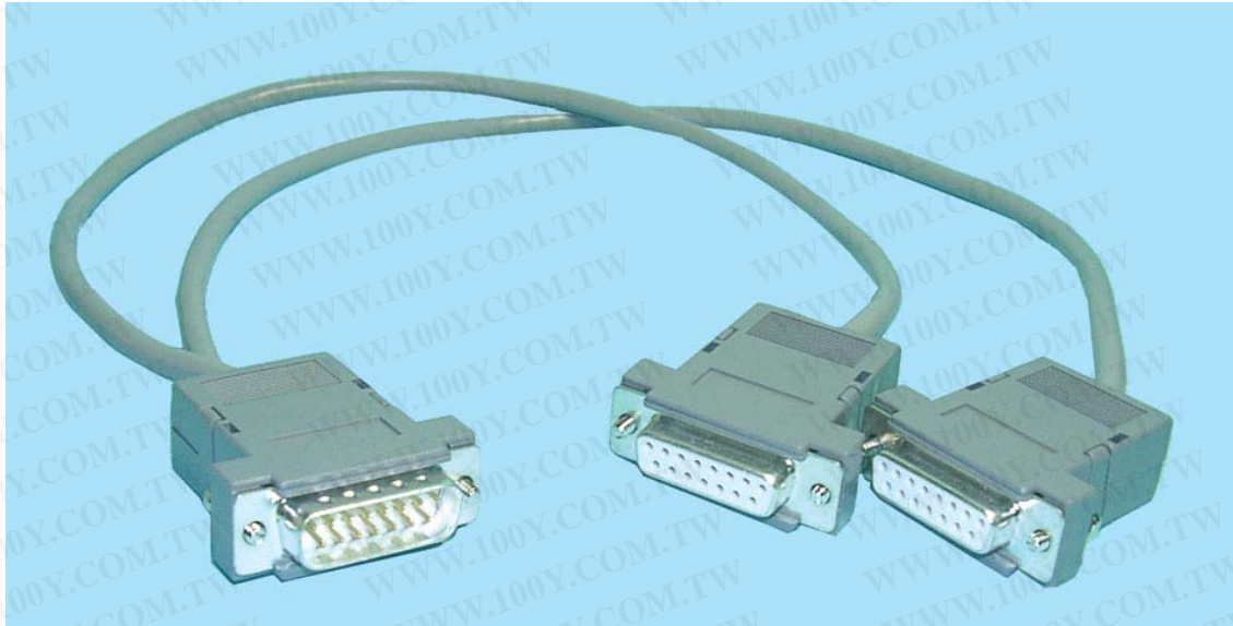
RS-232 15P Extension Cable
