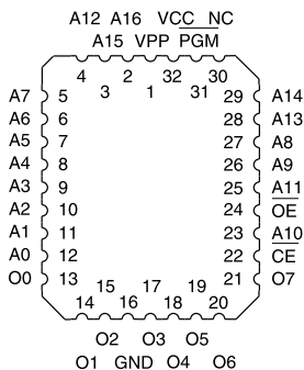
PLCC Top View
