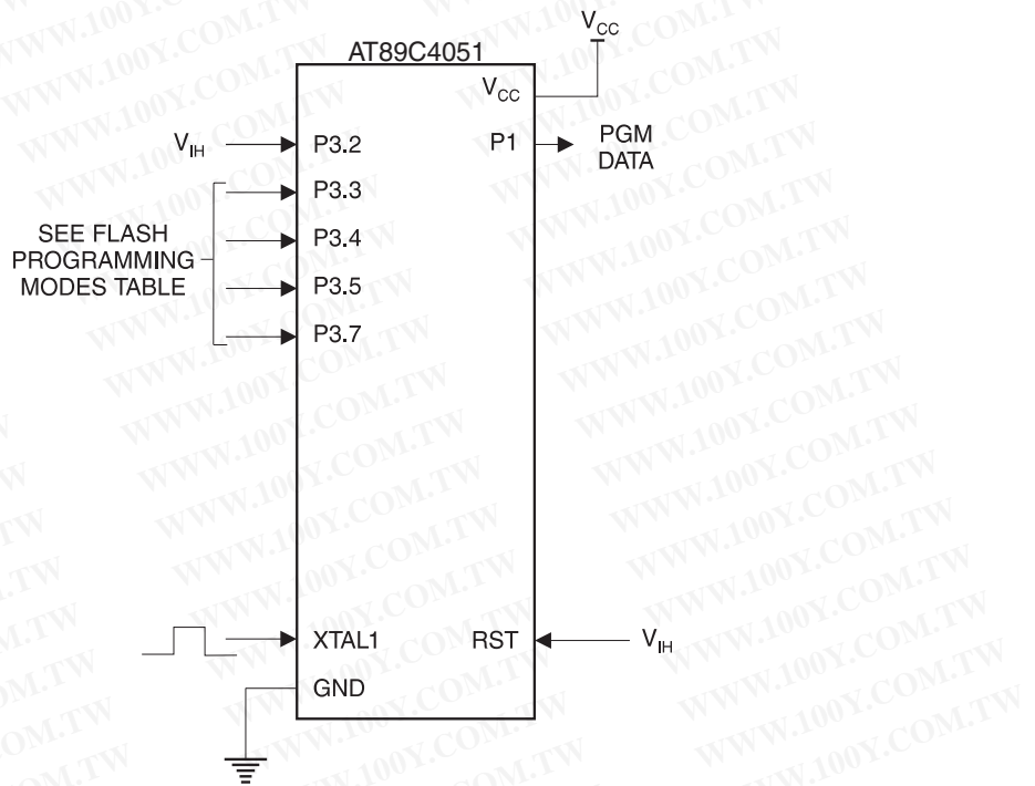
Figure 13-2. Verifying the Flash Memory
