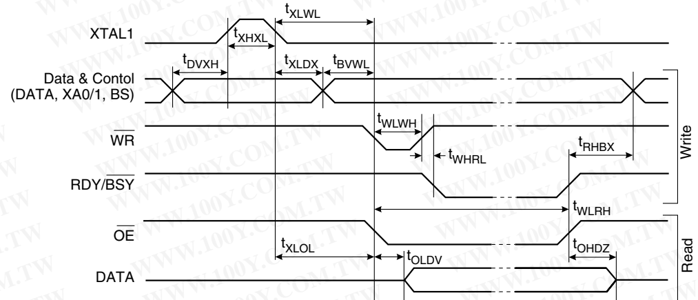
Figure 33. Parallel Programming Timing
