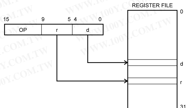
Figure 8. Direct Register Addressing, Two Registers
