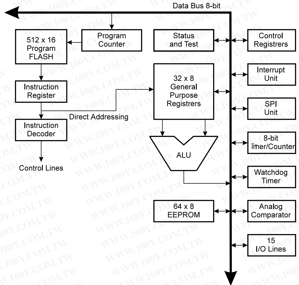
Figure 4. The AT90S1200 AVR RISC Architecture
