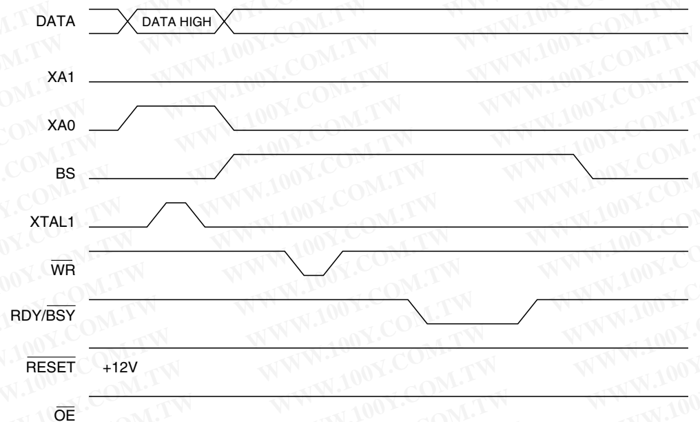
Figure 32. Programming the Flash Waveforms (Continued)
