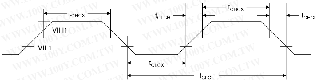
Figure 37. External Clock Drive
